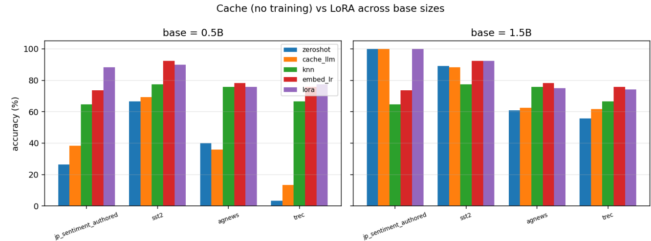
FIGURE 2. Cache versus LoRA at two base sizes (Qwen2.5-0.5B and 1.5B). Training-free embed+LR matches or beats LoRA on most tasks; the LLM path is competitive only at 1.5B.
