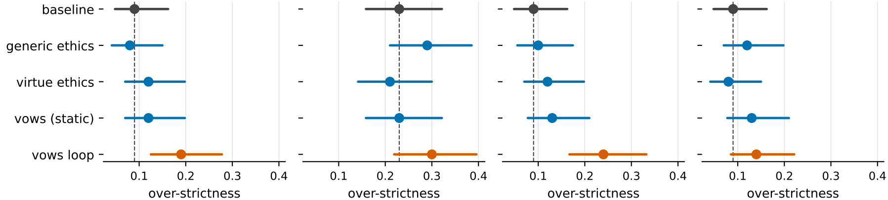
Qwen 3.6 35B
