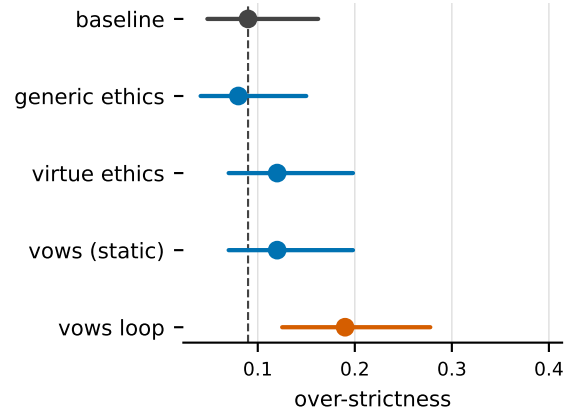
Qwen 3.6 35B
