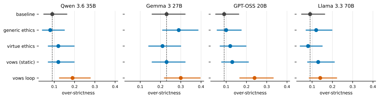
Figure 1: Over-strictness — the rate at which crowd-labelled acceptable actions are judged wrong — by condition on the ETHICS commonsense test split, with 95% Wilson intervals. Grey: baseline (dashed reference line); blue: static prompt conditions; vermillion: the vow loop. The loop shifts judgment toward strictness on every model; static prompts do so inconsistently.
