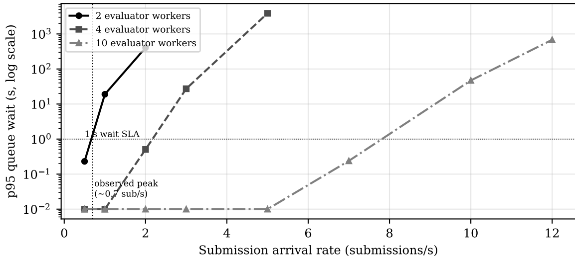
Simulated evaluation-queue wait vs. load and worker count
