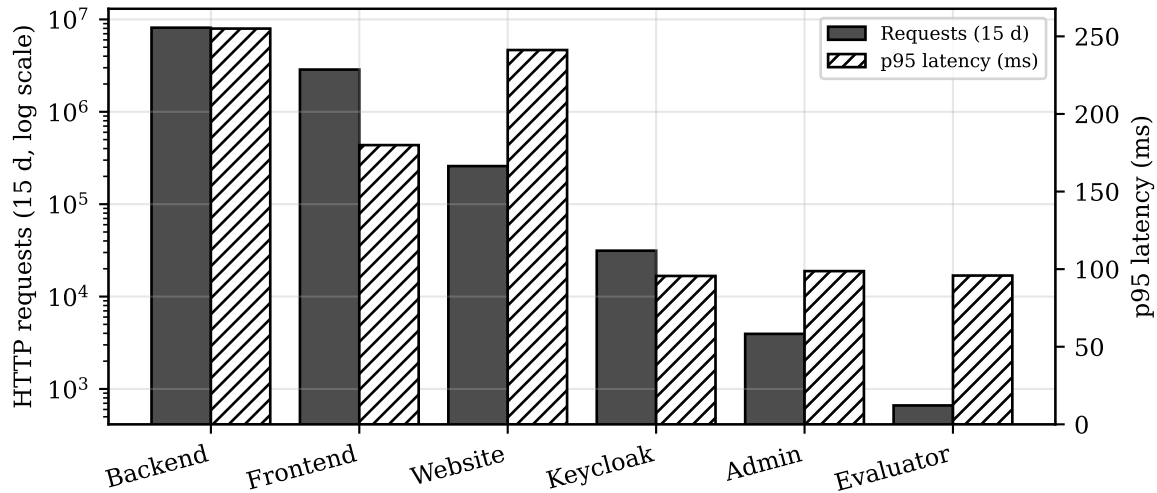
Per-service request volume and tail latency (steady state)
