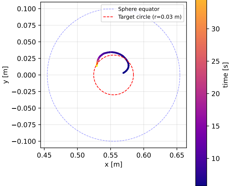
Tool Trajectory — Top View (XY Plane)
