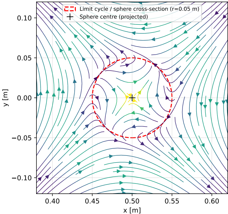
DS Velocity Field — Limit-Cycle Plane ( z = 0.4414 m)
