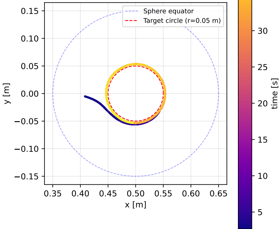
EE Trajectory — Top View (XY Plane)
