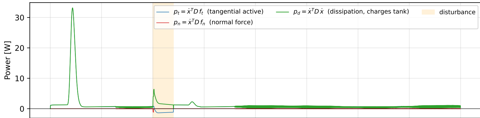
C. Power Terms ( p_d charges tank; p_t, p_n > 0 drain it)
