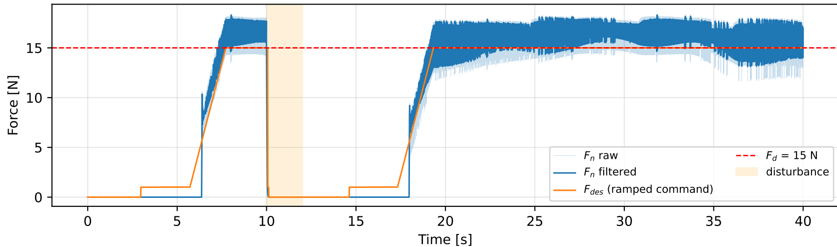
D. Contact Force Tracking
