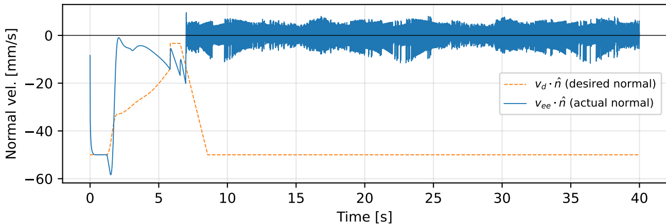
Normal Velocity (not tracked — converted to contact force by design)
