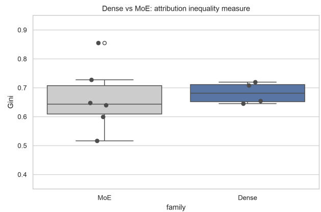
Figure 5: Dense vs. MoE Gini.
