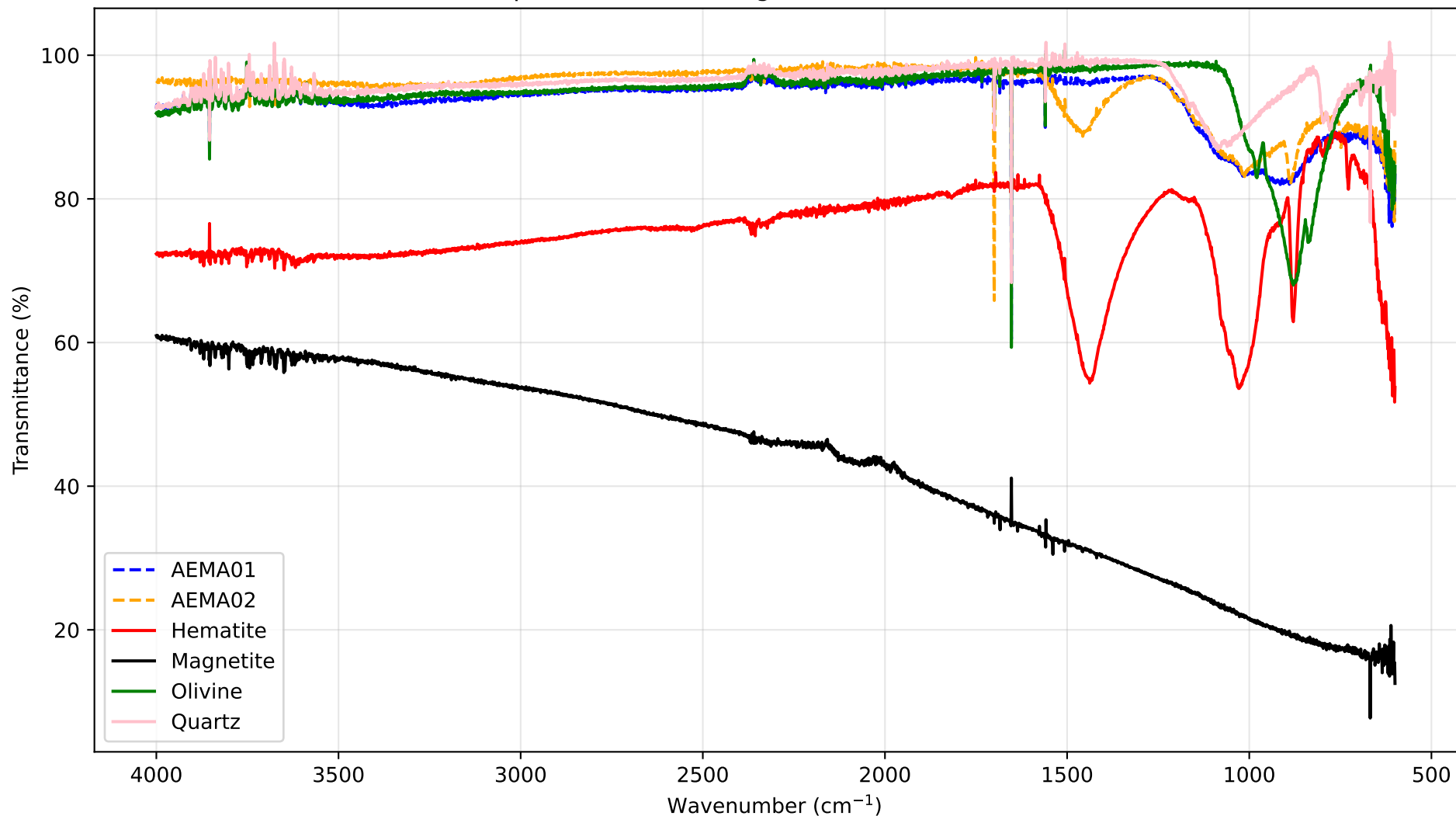
FTIR Spectra - Mars Analogues and Reference Minerals
