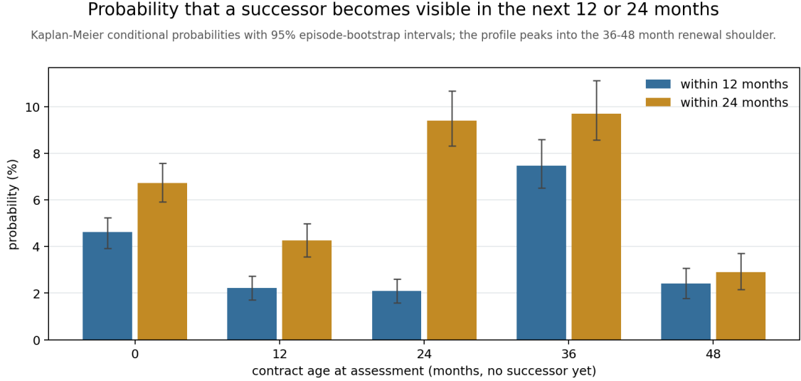
Figure 6: The same quantities with their bootstrap intervals. The profile is not monotone in age: it rises into the 36–48 month renewal shoulder and falls away after it, which is the empirical feature every parametric family smooths out.
