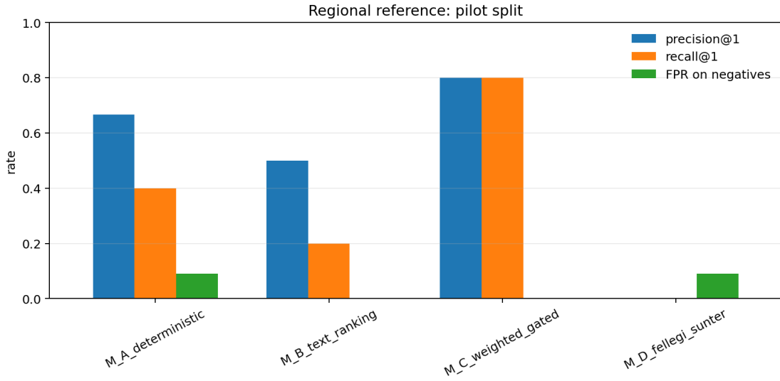
Figure 1: Pilot split method comparison generated from the regional-reference evaluation JSON.
