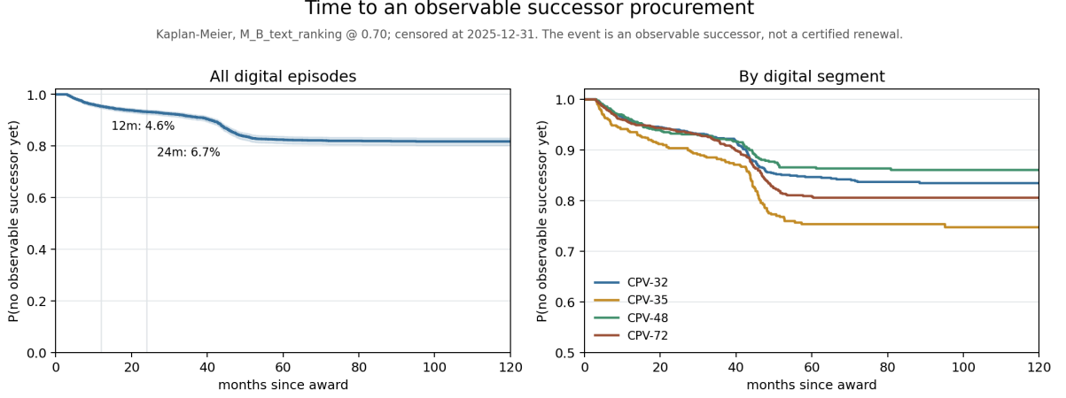
Figure 5: Kaplan–Meier survivor functions. The left panel carries the absolute level, which is linkage-conditioned and quoted only with that caveat; the right panel carries the segment ordering, which survives every sensitivity arm.
