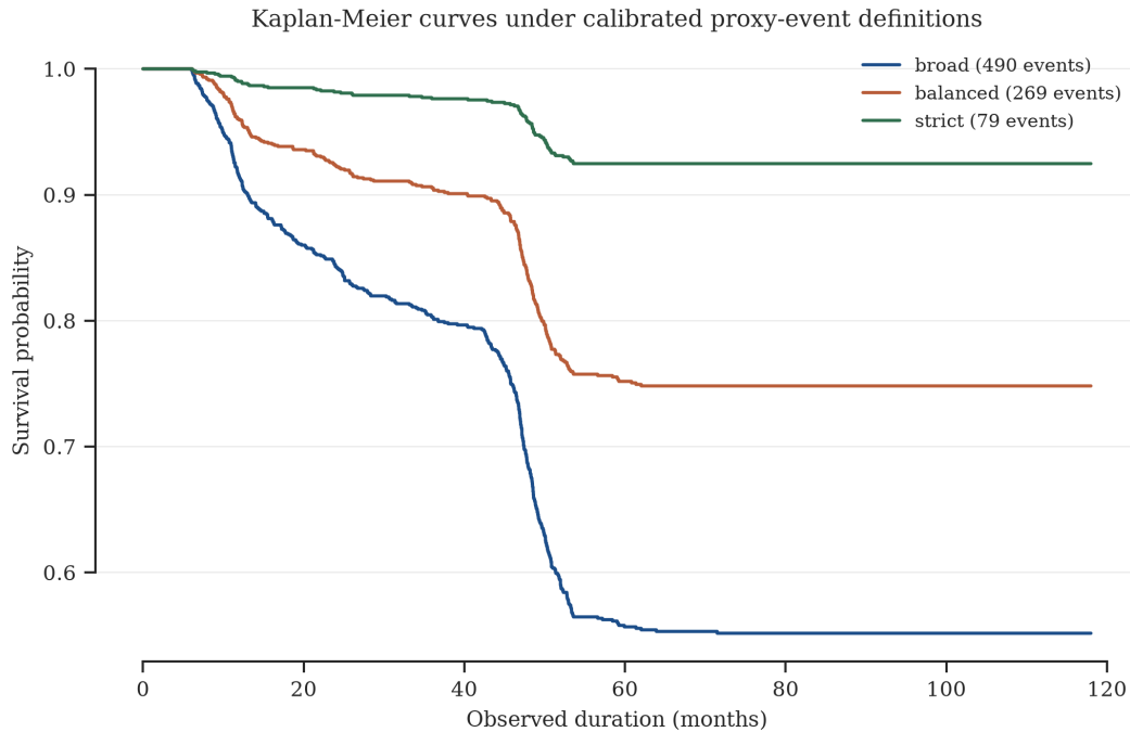
Figure 3: Kaplan–Meier survival curves under the three calibrated proxy-event rules. Stricter rules yield fewer, later-recorded events and higher residual survival at every horizon; the balanced curve sits between the broad and strict extremes, consistent with its intermediate event count.
