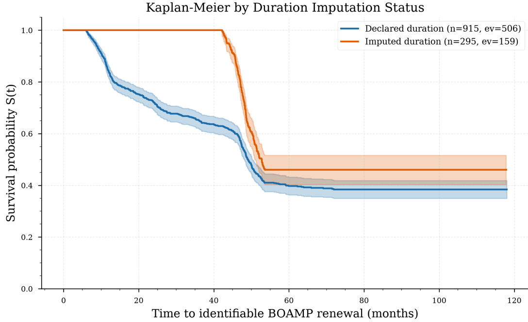
Figure 15: Kaplan–Meier survival curves by duration imputation status. Log-rank test: \chi^2 = 24.58 , p \approx 0 , df = 1 . Contracts with imputed durations (48-month default) renew later than those with observed durations.
