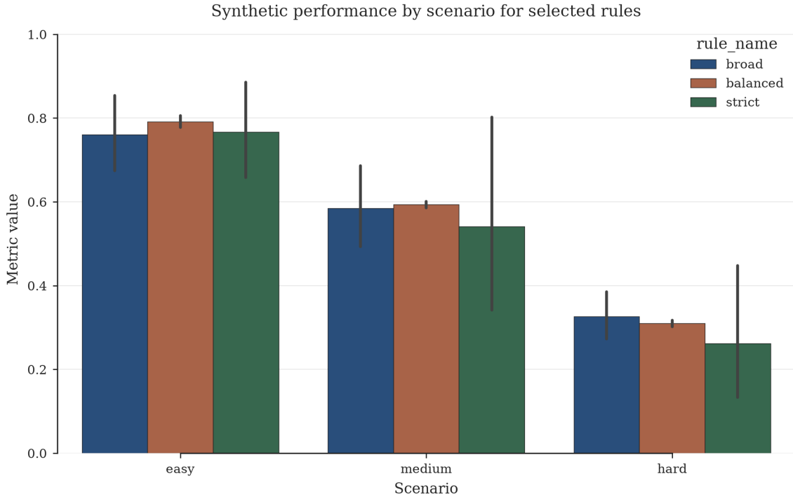
Figure 1: Synthetic-benchmark performance of the broad, balanced, and strict rules across the easy/medium/hard scenarios. All three rules degrade under harder synthetic noise, which is the intended stress test; the balanced rule was retained for its stability across scenarios rather than for being the single most precise option on paper.
