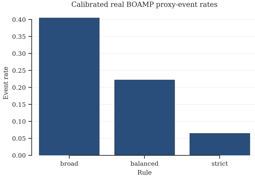
Figure 2: Proxy-event rate on real BOAMP under the three calibrated rules (1,210 eligible contracts). Moving from broad to balanced to strict trades linkage quantity for a rule whose behaviour has been checked on the synthetic benchmark above.
