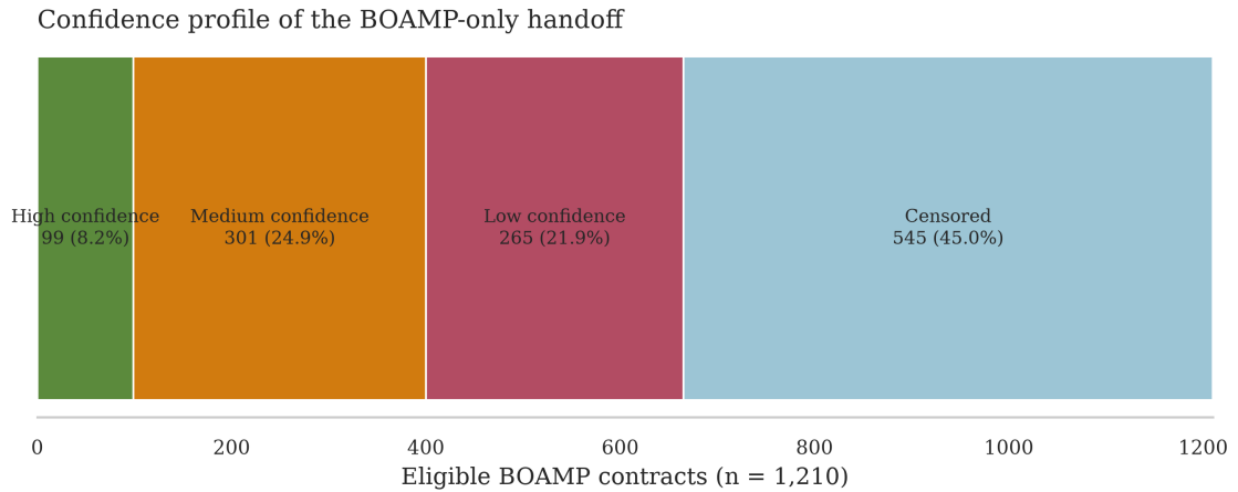
Figure 9: Confidence tier breakdown across all 1,210 eligible contracts. Green = HIGH ( S \geq 0.70 , n = 99 ); orange = MEDIUM ( 0.50 \leq S < 0.70 , n = 301 ); red = LOW ( S < 0.50 , n = 265 ); light blue = censored (event = 0, n = 545 ). The HIGH and MEDIUM tiers together cover 400 of the 665 linked contracts (60.2%), providing a reliable core dataset for survival modeling. LOW-tier links represent the greatest false-positive risk and should be downgraded to censored in the sensitivity check.
