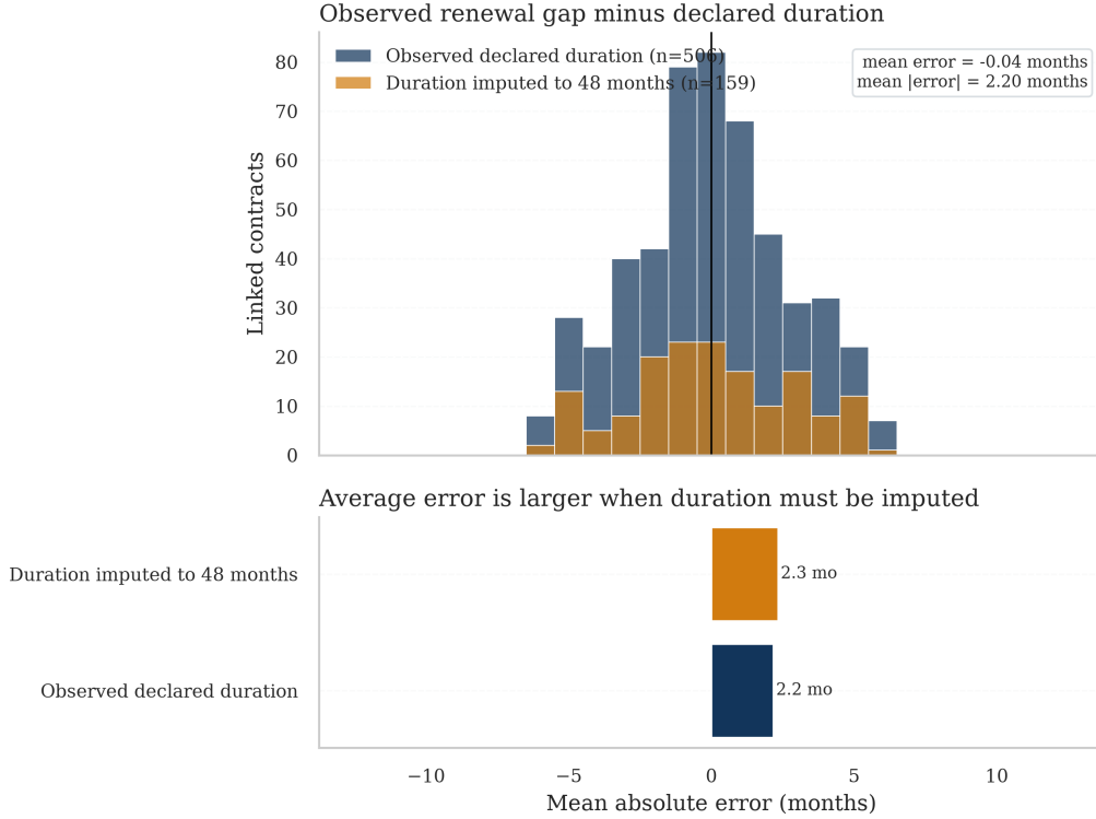
Figure 6: Distribution of the temporal error g(i, j^*) - d_i (observed gap minus declared duration) for the 665 linked contracts. Blue bars correspond to the 506 contracts with a valid non-imputed duration; orange bars to the 159 contracts whose duration was imputed to 48 months. The overall mean error is -0.04 months (effectively zero bias) with a standard deviation of 2.76 months. All pairs fall within \pm 6 months by construction of the hard filter, but the near-zero mean is consistent with the absence of a systematic temporal shift in the matches, though it cannot rule out residual bias from unobserved confounders. Imputed-duration contracts show a similar spread (mean |\text{error}| = 2.3 vs. 2.2 months for non-imputed).
