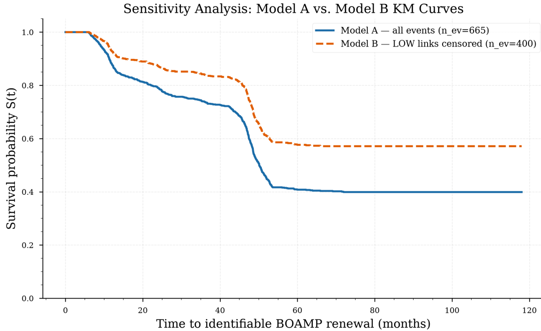
Figure 19: Kaplan–Meier comparison: Model A (all 665 linked contracts, median 50.1 mo) vs. Model B (400 high/medium-confidence contracts, median not reached). The two curves share broadly consistent shapes; the Model B curve sits higher because 265 LOW-tier links are downgraded to censored. The Cox concordance (0.632 vs. 0.616) suggests that lower-confidence links add noise but do not appear to introduce a dominant systematic bias in the ranking of renewal risk.
