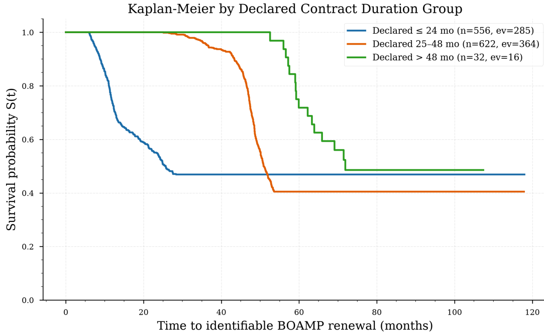
Figure 14: Kaplan–Meier survival curves stratified by declared duration group ( \leq 24 mo, 25–48 mo, > 48 mo). Log-rank test: \chi^2 = 62.30 , p \approx 0 , df = 2 . Shorter declared durations are associated with earlier renewal events.
