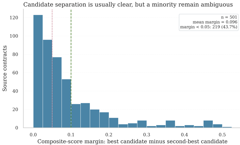
Figure 11: Distribution of the score margin m_i (best composite – second-best composite) for the 501 multi-candidate source contracts. The dotted red line marks the 0.05 threshold below which 43.7% of pairs are considered ambiguous : the algorithm selected one candidate, but an alternative was within 0.05 of the same score. The dashed green line at 0.10 marks the clear winner zone (30.3% of pairs). These ambiguous pairs are concentrated in the LOW and MEDIUM confidence tiers and are the primary motivation for the manual validation sample recommended in Section 11.
