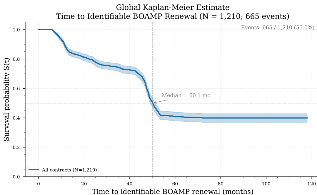
Figure 12: Global Kaplan–Meier survival curve for all 1,210 eligible contracts. The solid blue line is the KM estimate; the shaded band is the 95% pointwise confidence interval. Censored observations are marked by tick marks. Median survival = 50.1 months (vertical dashed line).
