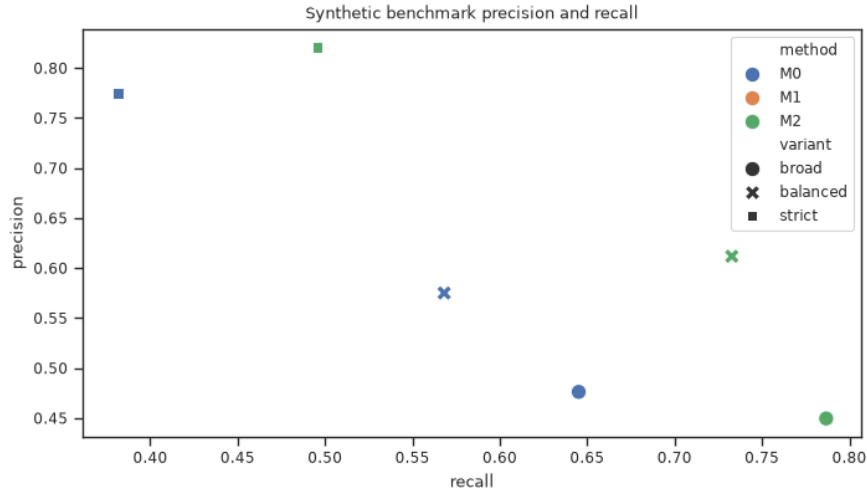
Figure 4: Synthetic benchmark-estimated precision and recall for M0, M1, and M2. The synthetic benchmark supports comparing methods, but it does not prove real BOAMP truth.
