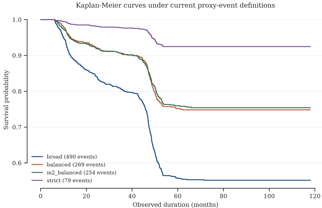
Figure 3: Kaplan–Meier survival curves under the current proxy-event definitions (M0 broad/balanced/strict and the selected M2 balanced). The stricter the rule, the fewer and later the recorded events, and the higher the residual survival at any horizon; the M2 balanced curve tracks the M0 balanced curve closely.
