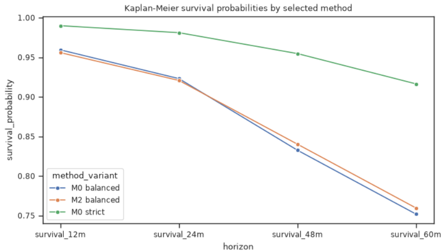
Figure 5: Fixed-horizon Kaplan–Meier survival probabilities for M0 balanced, M2 balanced, and M0 strict. M2 balanced is the selected main method; its survival profile is close to the M0 balanced baseline.
