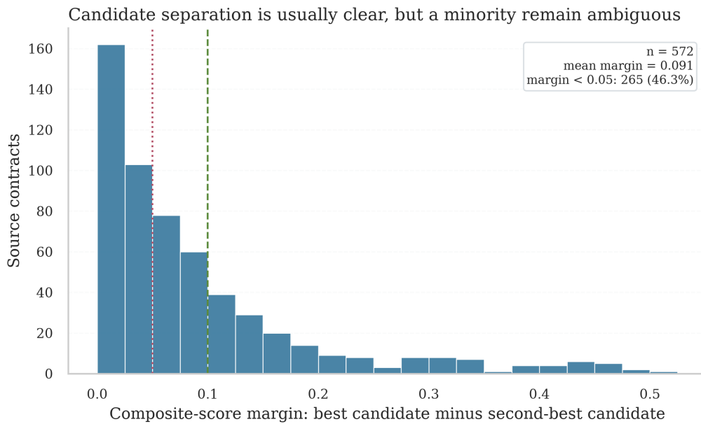
Figure 8: Distribution of the score margin m_i (best composite – second-best composite) for the 572 multi-candidate source contracts. The dotted red line marks the 0.05 threshold below which 46.3% of pairs are considered ambiguous : the algorithm selected one candidate, but an alternative was within 0.05 of the same score. The dashed green line at 0.10 marks the clear winner zone (29.5% of pairs). These ambiguous pairs are concentrated in the LOW and MEDIUM confidence tiers and are the primary motivation for the manual validation sample recommended in Section 11.
