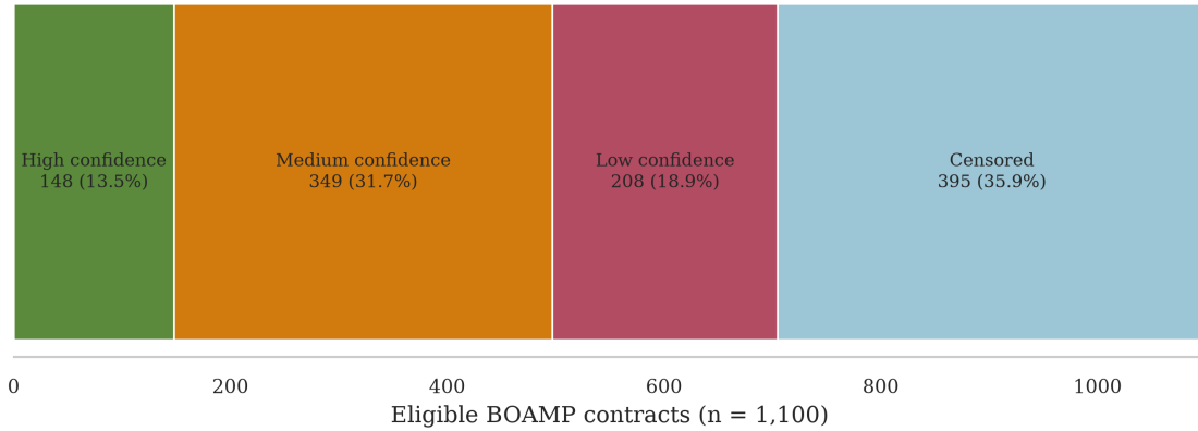
Figure 6: Confidence tier breakdown across all 1,100 eligible contracts. Green = HIGH ( S \geq 0.70 , n = 148 ); orange = MEDIUM ( 0.50 \leq S < 0.70 , n = 349 ); red = LOW ( S < 0.50 , n = 208 ); light blue = censored (event = 0, n = 395 ). The HIGH and MEDIUM tiers together cover 497 of the 705 linked contracts (70.5%), providing a reliable core dataset for survival modeling. LOW-tier links represent the greatest false-positive risk and should be downgraded to censored in the sensitivity check.
