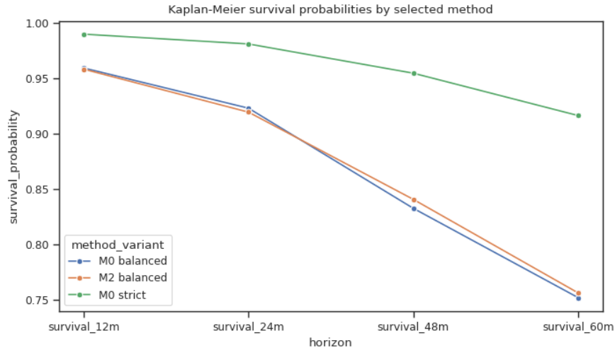
Figure 5: Fixed-horizon Kaplan–Meier survival probabilities for M0 balanced, M2 balanced, and M0 strict. M0 balanced remains the selected method.
