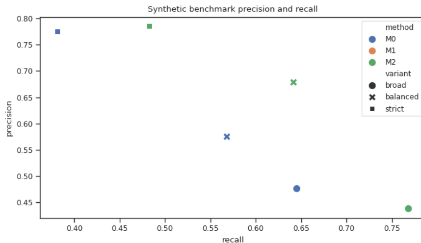
Figure 4: Synthetic precision and recall for M0, M1, and M2. The synthetic benchmark supports comparing methods, but it does not prove real BOAMP truth.
