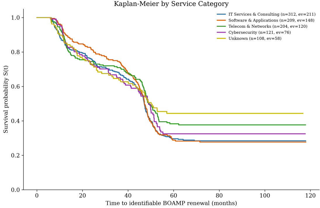
Figure 9: Kaplan–Meier survival curves stratified by service category. Log-rank test: \chi^2 = 6.23 , p = 0.182 , df = 4 . No category shows a statistically significant difference in time-to-renewal.
