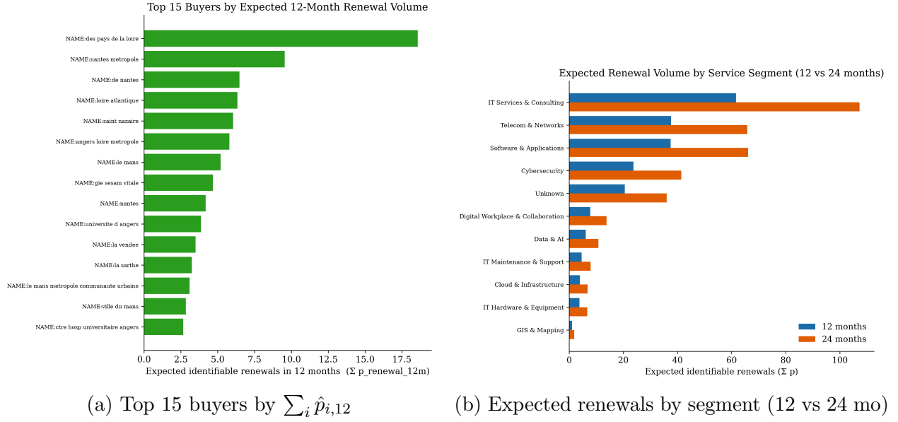
Figure 17: Operational renewal-risk rankings: buyers with the largest near-term expected renewal volume (left) and expected renewal volume by service segment (right).
