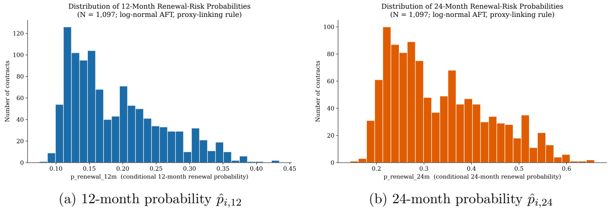
Figure 16: Distribution of contract-level renewal-risk probabilities under the log-normal AFT model (proxy-linking rule, N = 1,097 ).
