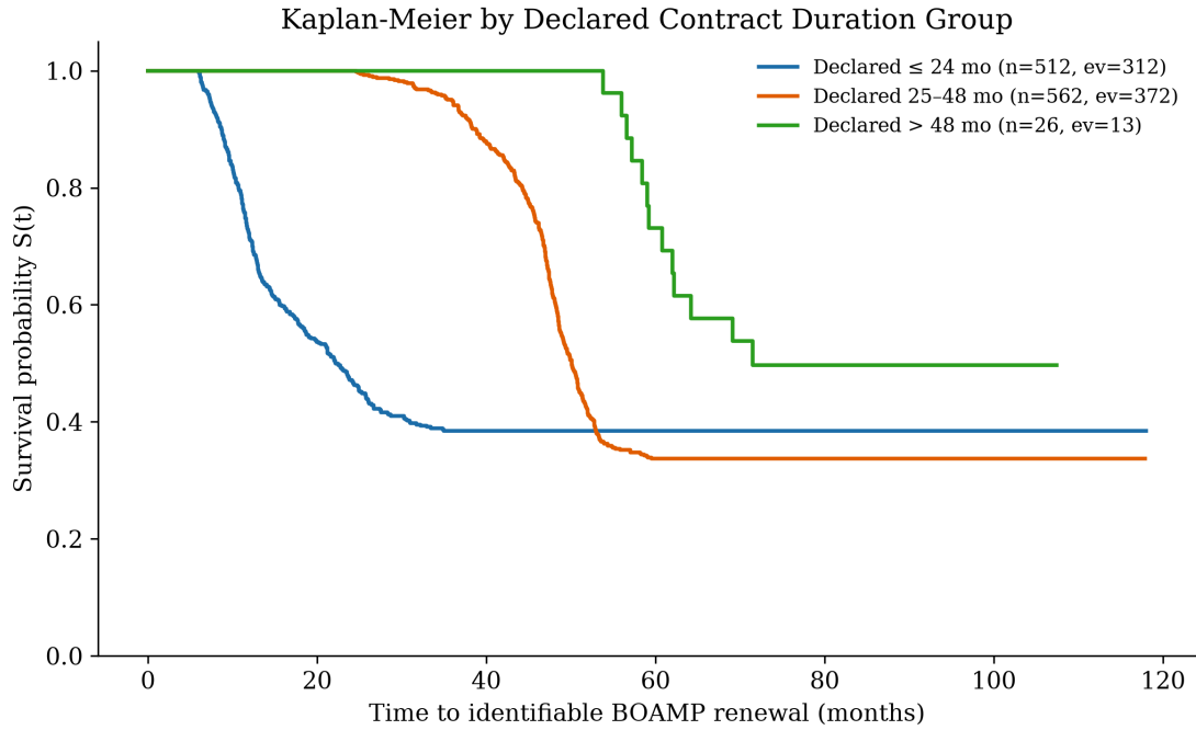
Figure 10: Kaplan–Meier survival curves stratified by declared duration group ( \leq 24 mo, 25–48 mo, > 48 mo). Log-rank test: \chi^2 = 62.30 , p \approx 0 , df = 2 . Shorter declared durations are associated with earlier renewal events.
