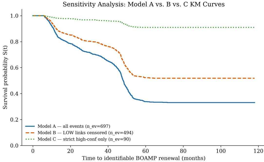
Figure 15: Kaplan–Meier comparison: Model A (all 697 linked contracts) vs. Model B (494 high/medium-confidence contracts) vs. Model C (90 strict high-confidence links). Models A and B share broadly consistent curve shapes; Model C sits far higher (most contracts censored), so its survival curve never reaches 0.5. The stable Cox concordance across all three confirms that lower-confidence links add noise but do not appear to introduce a dominant systematic bias in the ranking of renewal risk.
