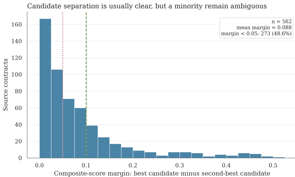
Figure 7: Distribution of the score margin (best composite – second-best composite) for the 562 multi-candidate source contracts. The dotted red line marks the 0.05 threshold below which 48.6% of pairs are considered ambiguous : the algorithm selected one candidate, but an alternative was within 0.05 of the same score. The dashed green line at 0.10 marks the clear winner zone (28.1% of pairs). These ambiguous pairs are concentrated in the LOW and MEDIUM confidence tiers and are the primary motivation for the manual validation sample recommended in Section 11.
