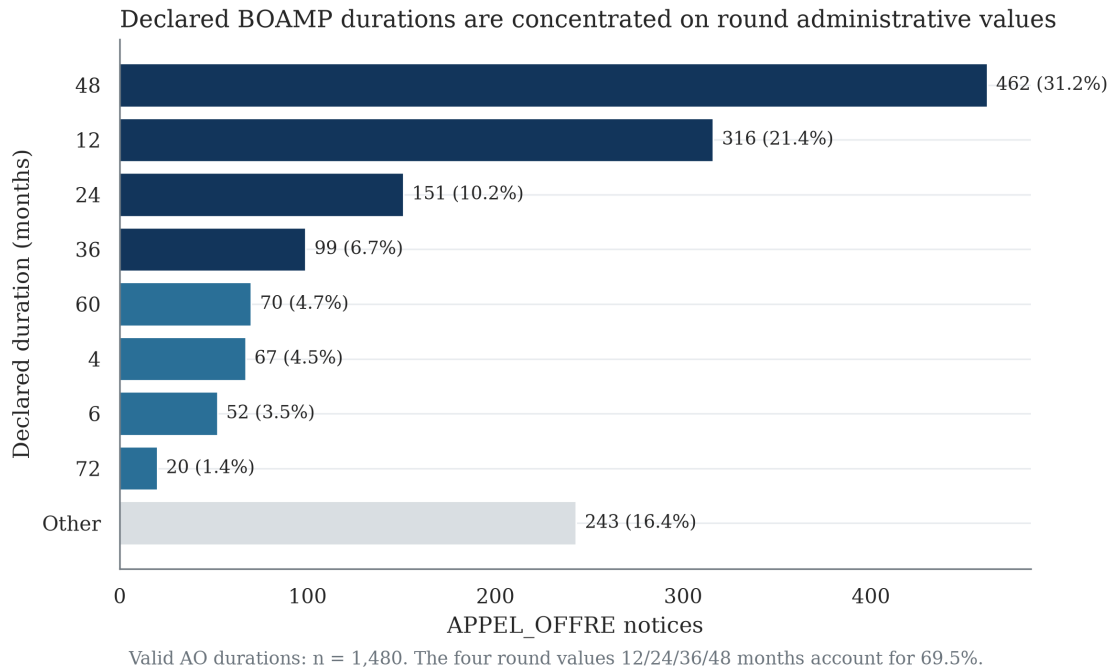
Figure 1: Distribution of declared duration values for the 1,480 APPEL_OFFRE notices with a valid duration_clean . Dark bars mark the four exact round values (12, 24, 36, 48 months) that together account for 69.5% of all valid durations. Light-blue bars are other specific values; grey is all remaining values combined. The concentration at round multiples of 12 reflects the administrative maximum declaration required by French procurement law, not empirically measured contract lifetimes.
