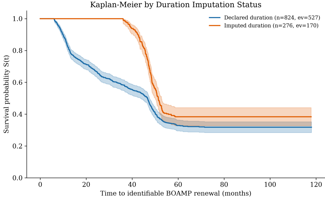
Figure 11: Kaplan–Meier survival curves by duration imputation status. Log-rank test: \chi^2 = 24.58 , p \approx 0 , df = 1 . Contracts with imputed durations (48-month default) renew later than those with observed durations.
