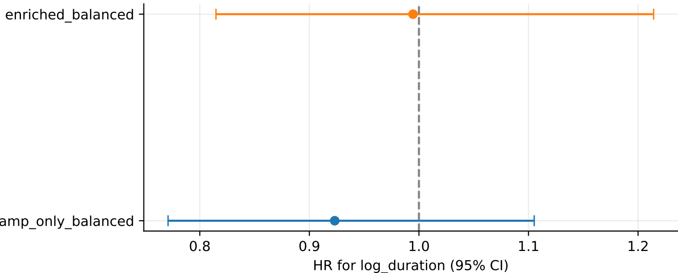
Duration hazard ratio by layer
