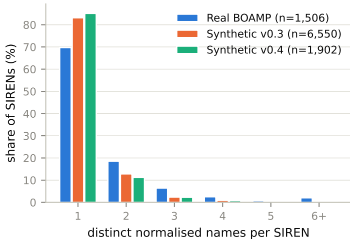
Alias-set size distribution
