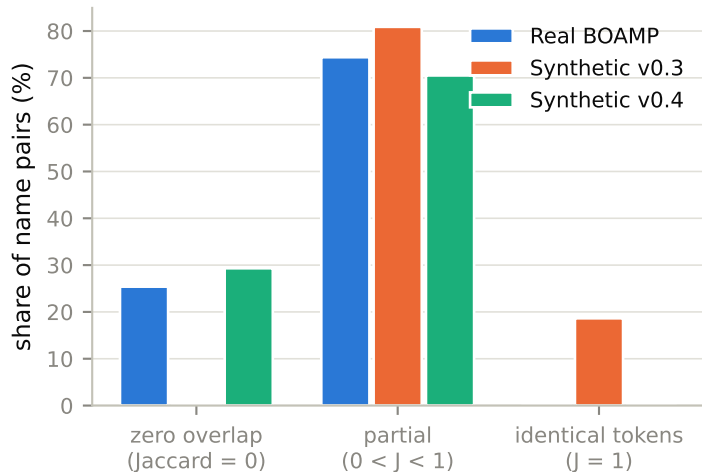
Overlap bands: before vs after the alias mechanism
