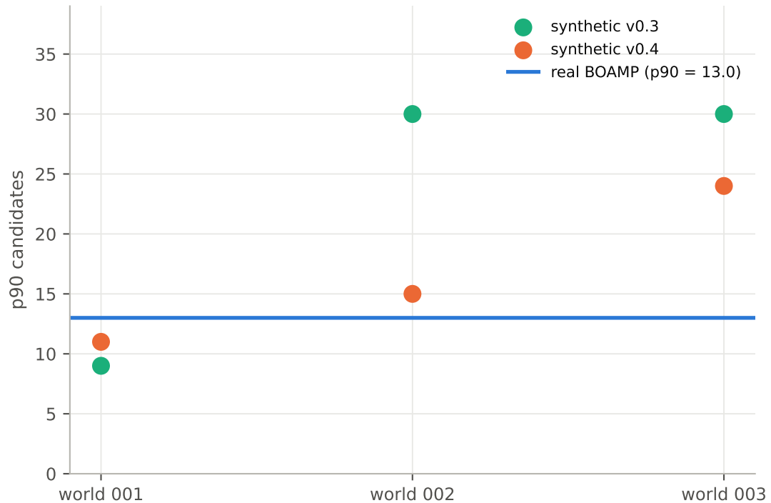
(b) p90 candidates per source, by world and version
