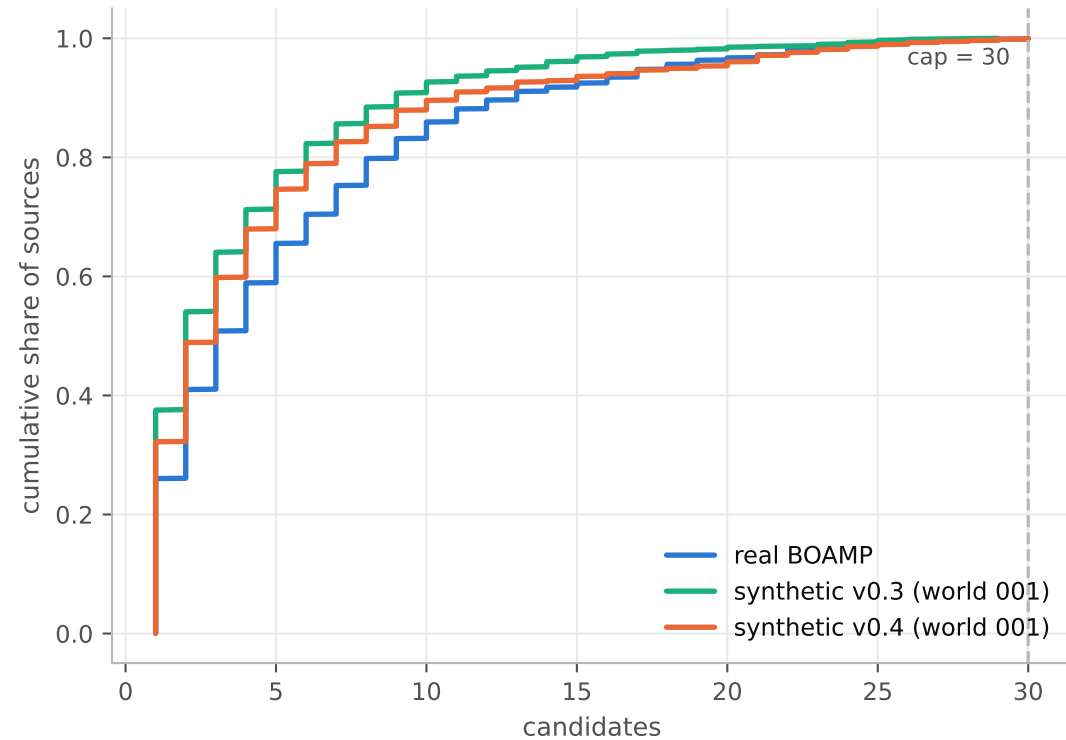
(a) Candidates generated per source
