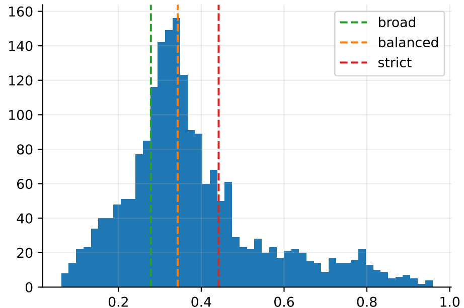
L1 rank-1 composite score with frozen thresholds
