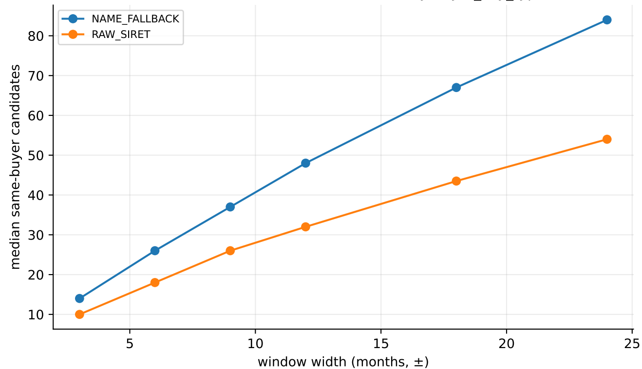
Candidate-set size vs. window width, by buyer_key_type
