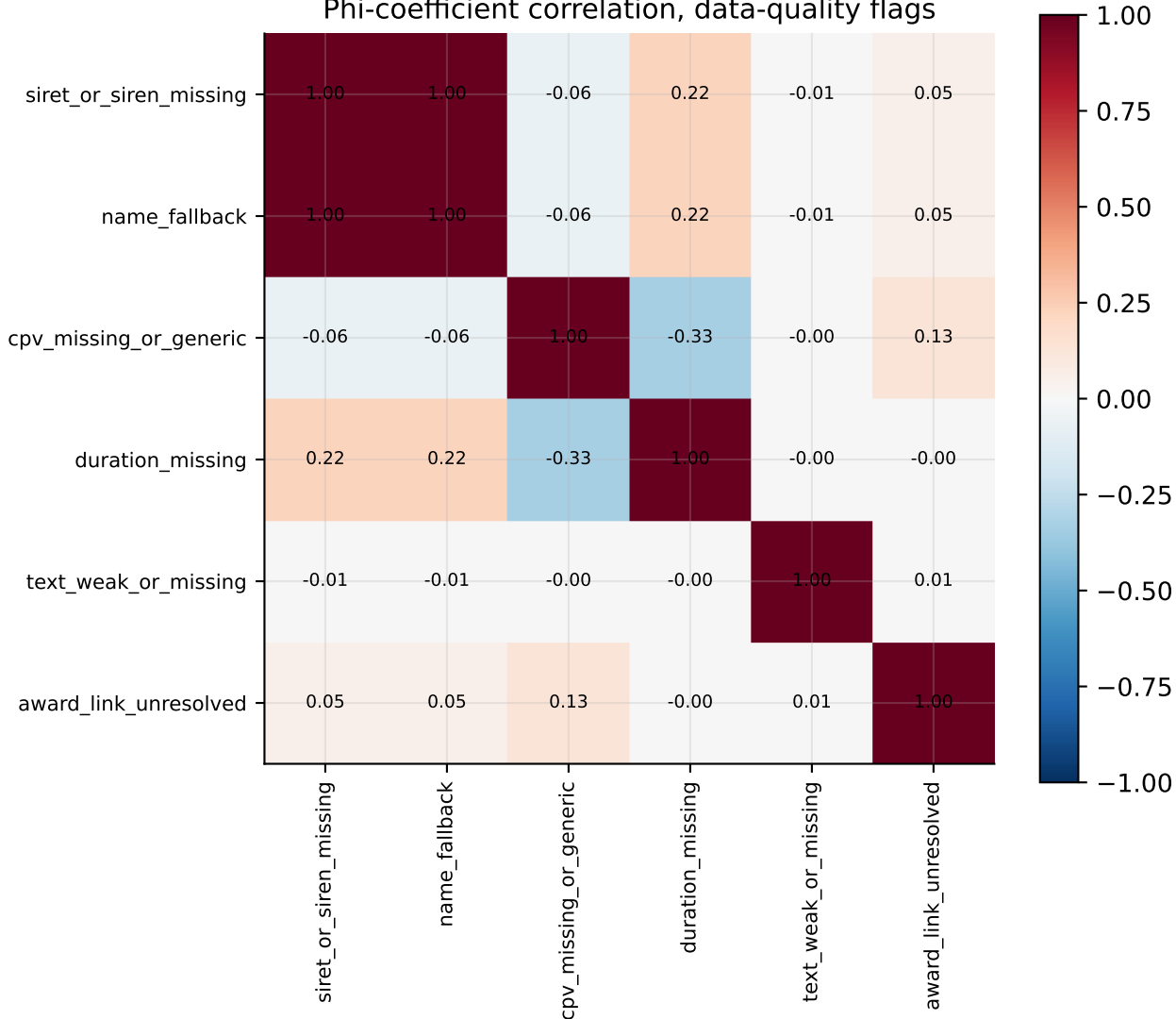
Phi-coefficient correlation, data-quality flags
