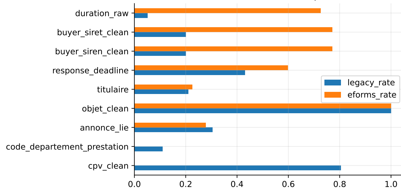
LEGACY vs EFORMS field completeness
