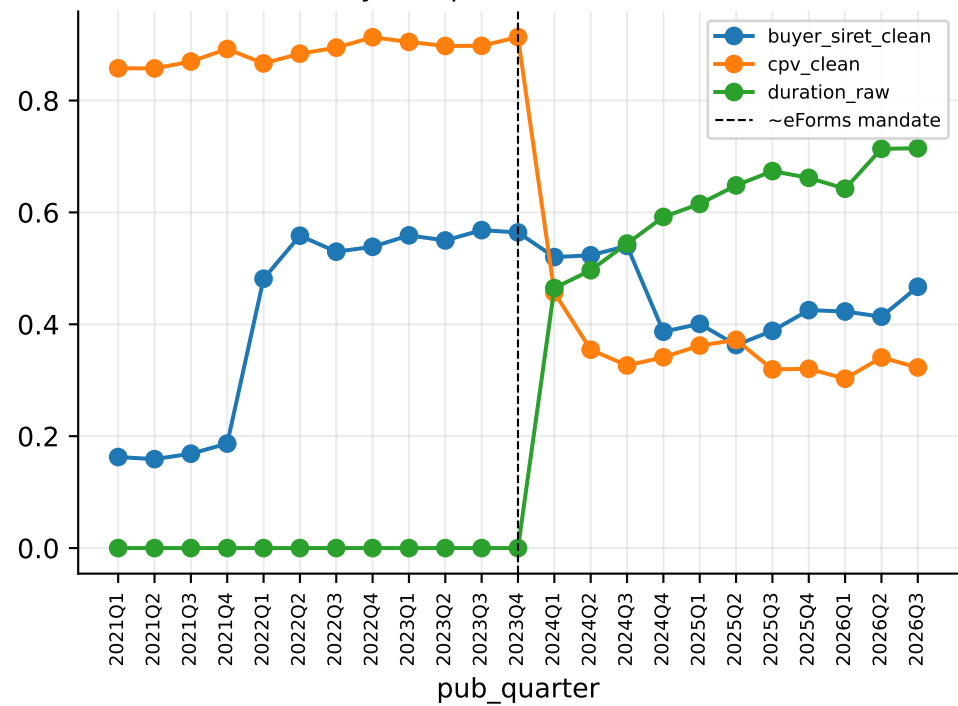
Quarterly completeness trend, 2021+
