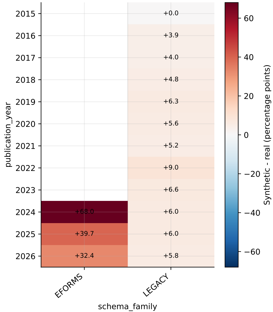
Duration present conditional difference | notice_type_normalized=ATtribution
