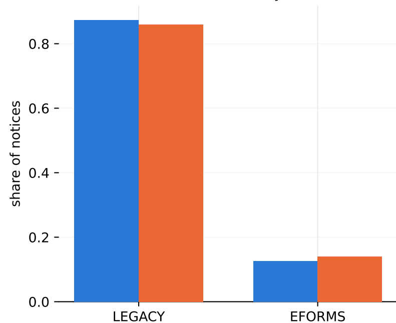
Schema family
