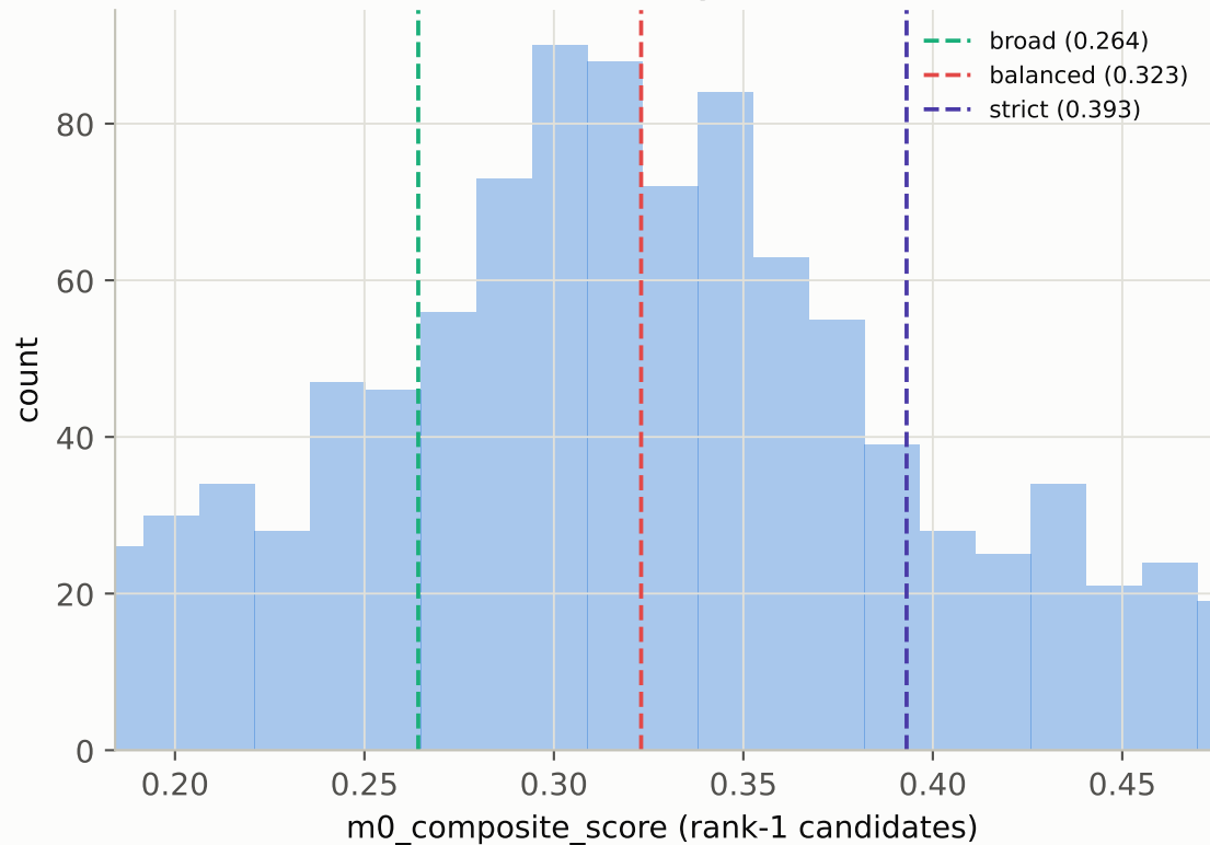
(b) local score density near thresholds
