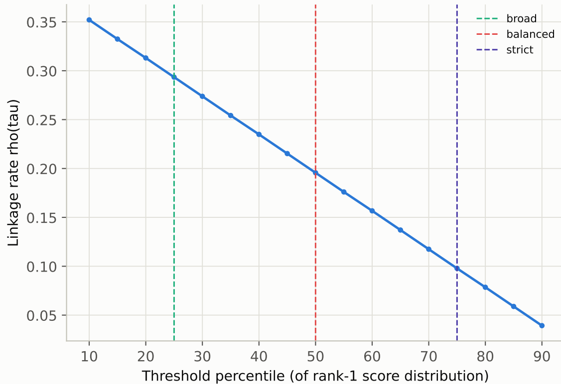
(a) rho(tau) sweep
