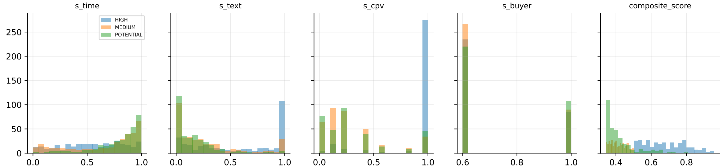
[balanced variant] component-score distributions by confidence tier [SILVER_STANDARD] Consistency check only; scores selected these links, so a well-behaved distribution here is not independent validation.
