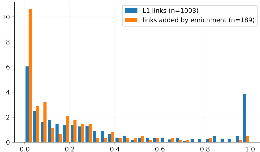
Text similarity: L1 links vs enrichment-added links (descriptive)
