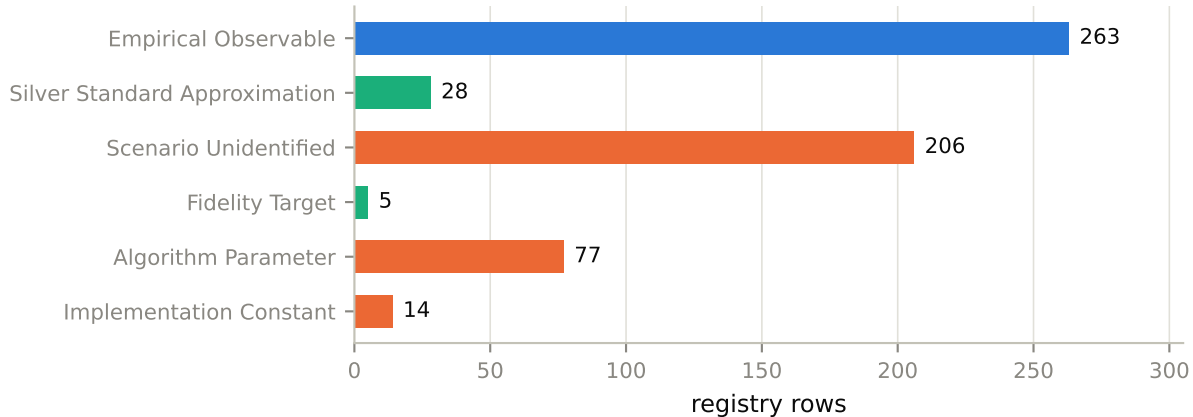
Provenance of every registered generator parameter and validation rule
