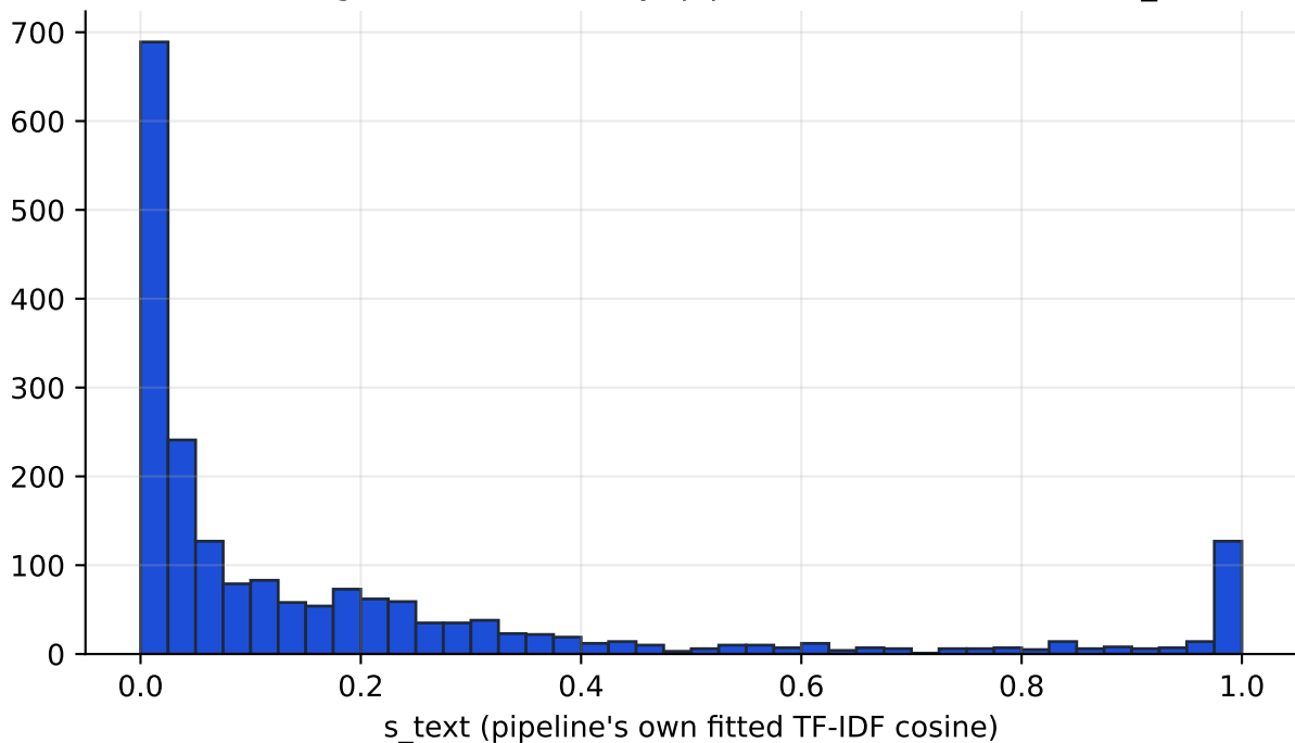
Nearest-neighbor text similarity (pipeline rank-1 candidates, s_text)
