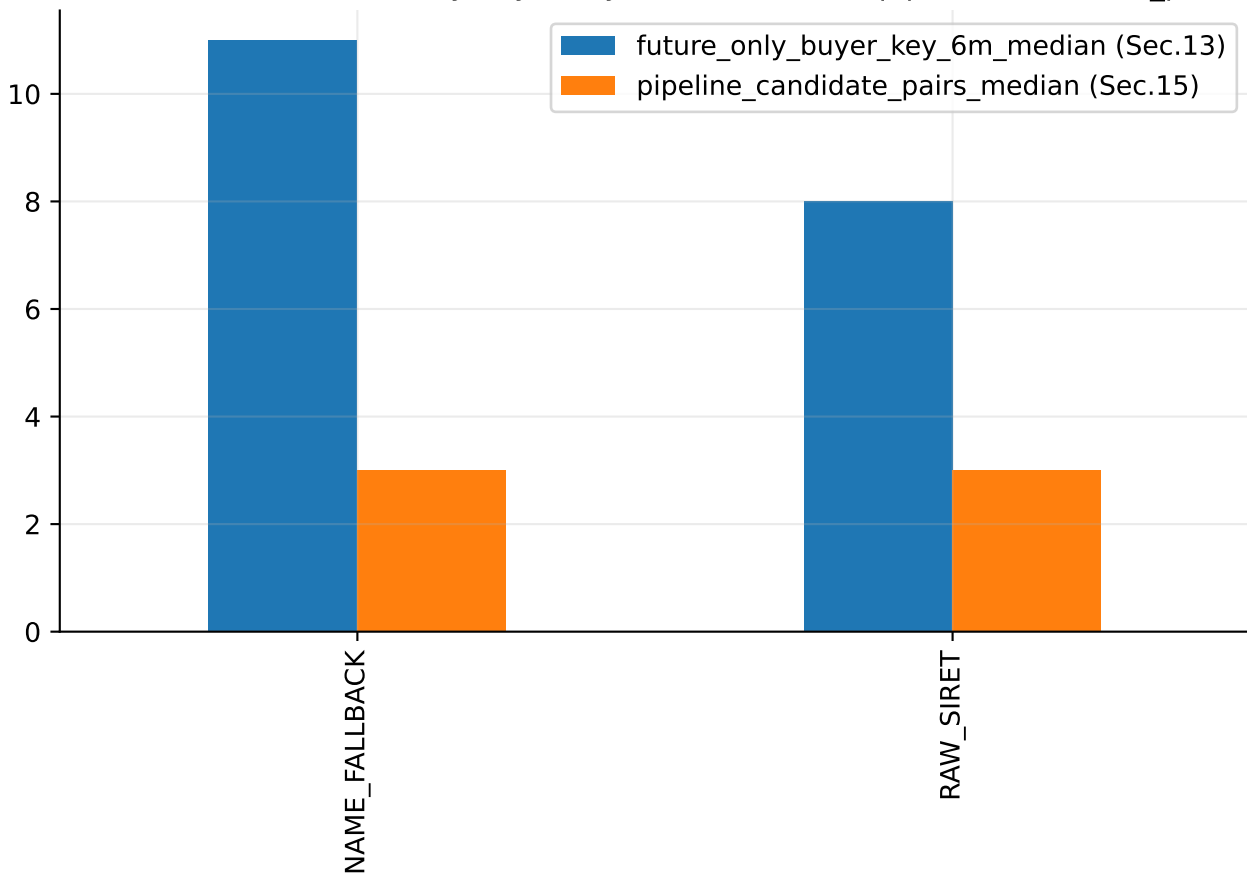
Candidate-set size: future-only buyer-key environment vs. pipeline candidate_pairs.csv
