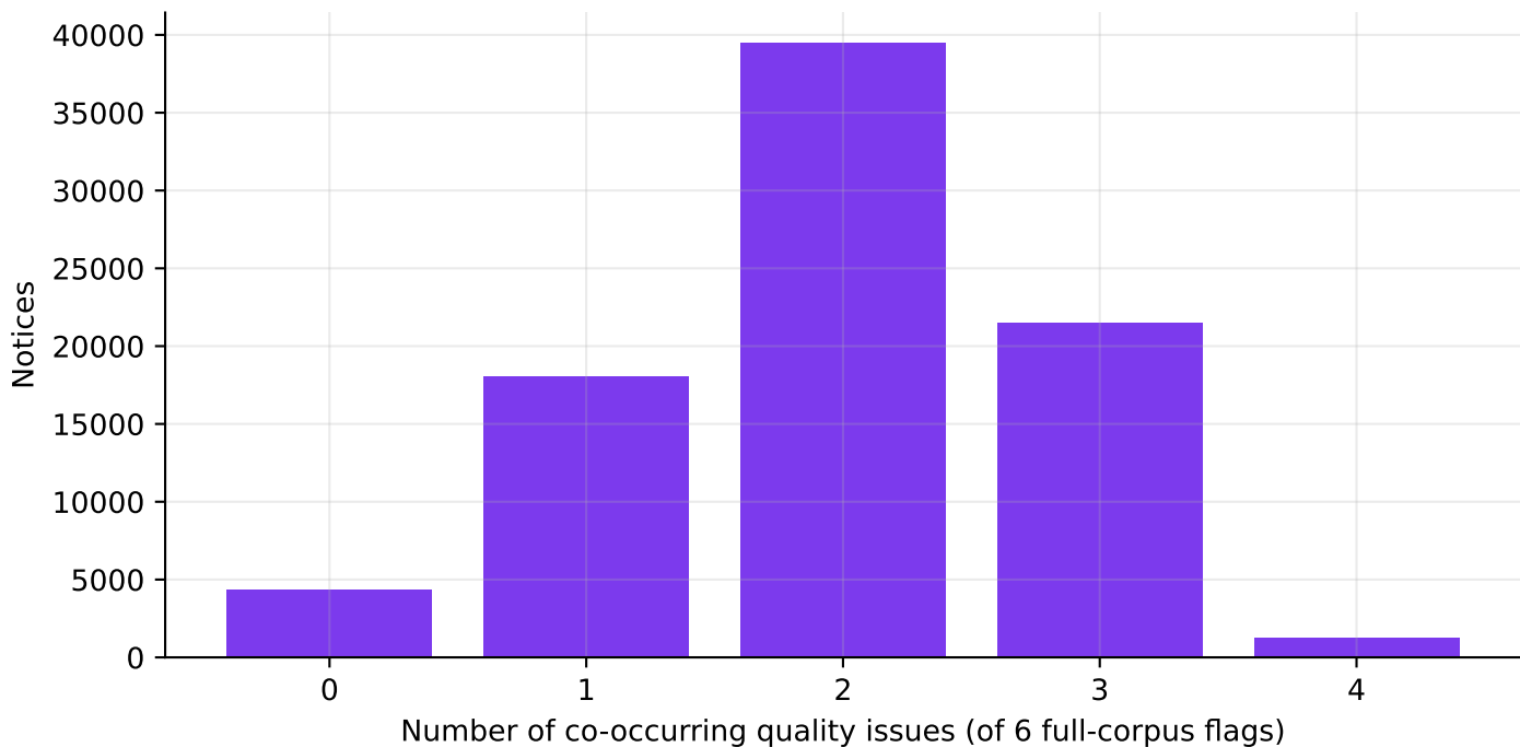
Issue-count distribution
