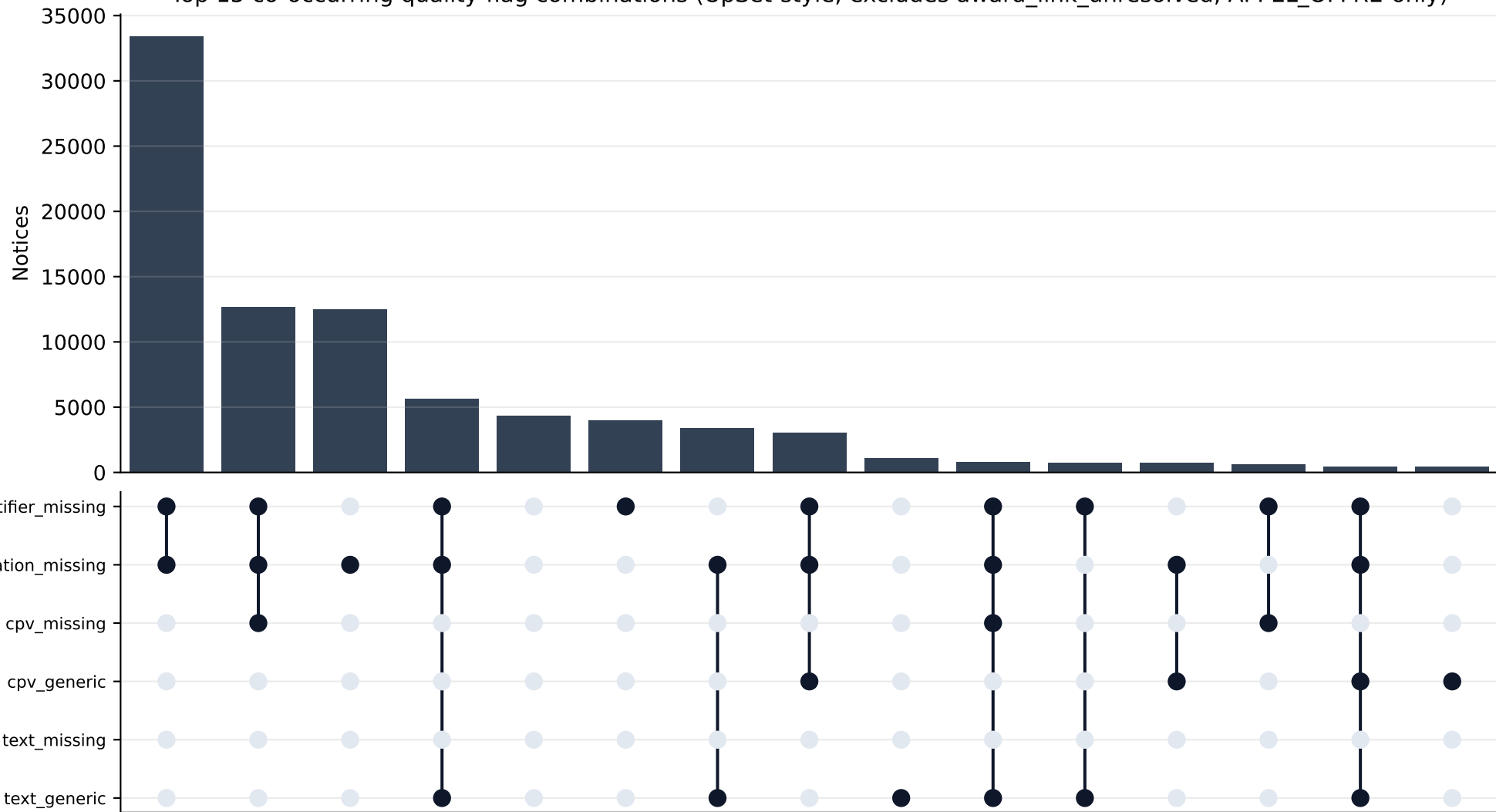
Top 15 co-occurring quality-flag combinations (UpSet-style; excludes award_link_unresolved, APPEL_OFFRE-only)
