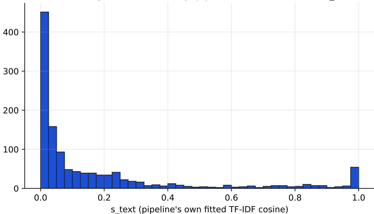
Nearest-neighbor text similarity (pipeline rank-1 candidates, s_{\text{text}} )
