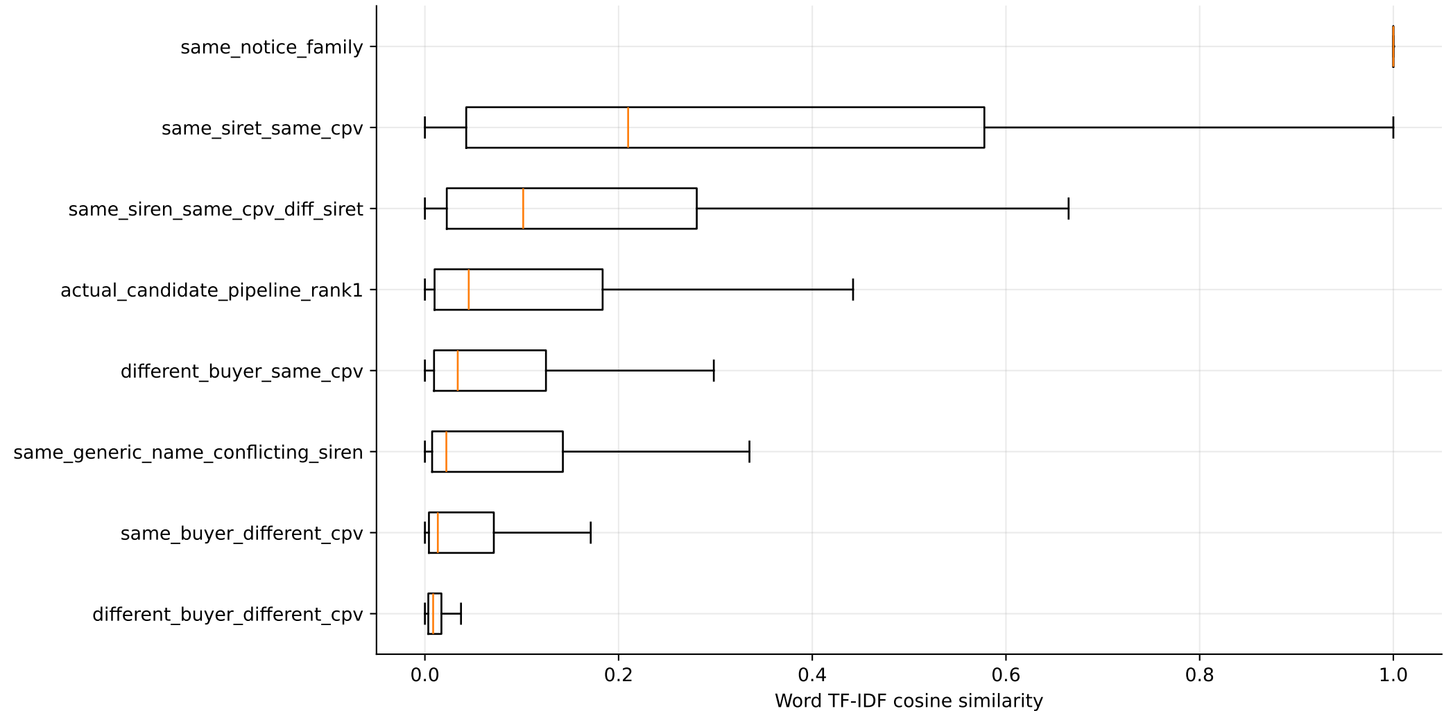
Text similarity distribution by pair group (Work Package 6)
