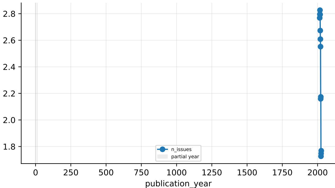
Mean number of co-occurring quality issues (of 5) per notice, by year
