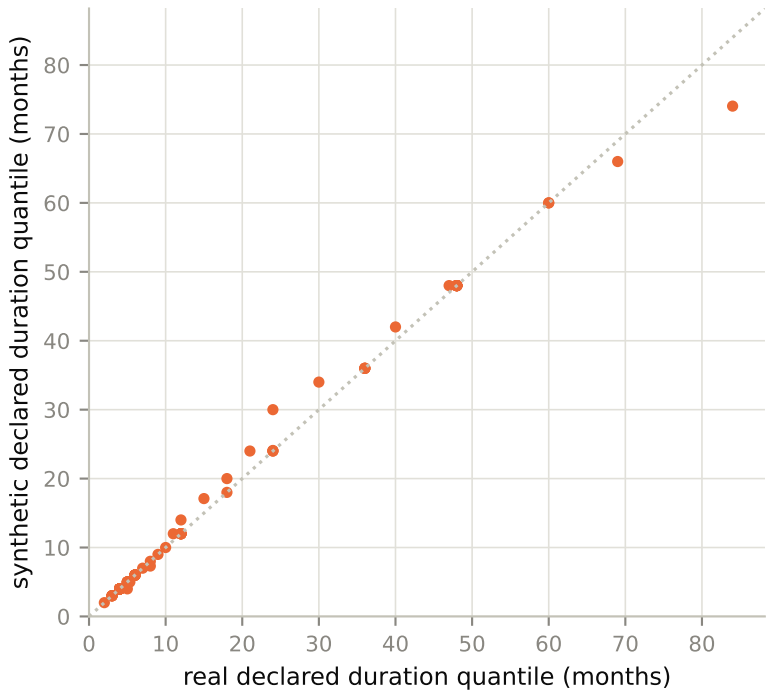
Declared-duration quantiles
