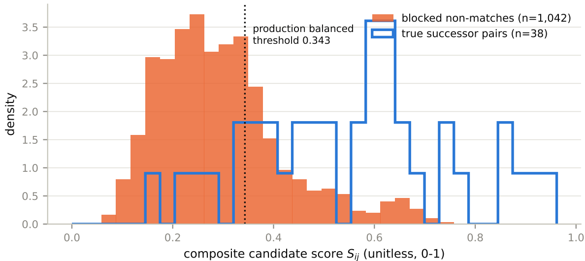
Score separability of sealed truth from same-buyer distractors
