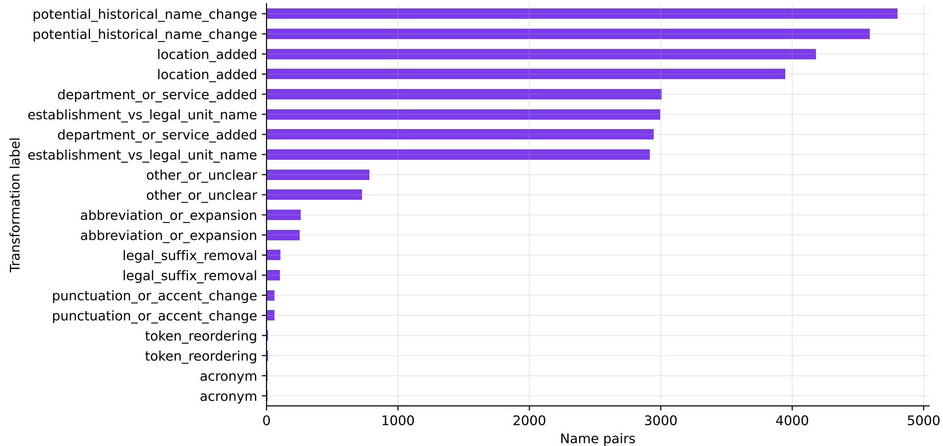
Likely buyer-name transformation labels
