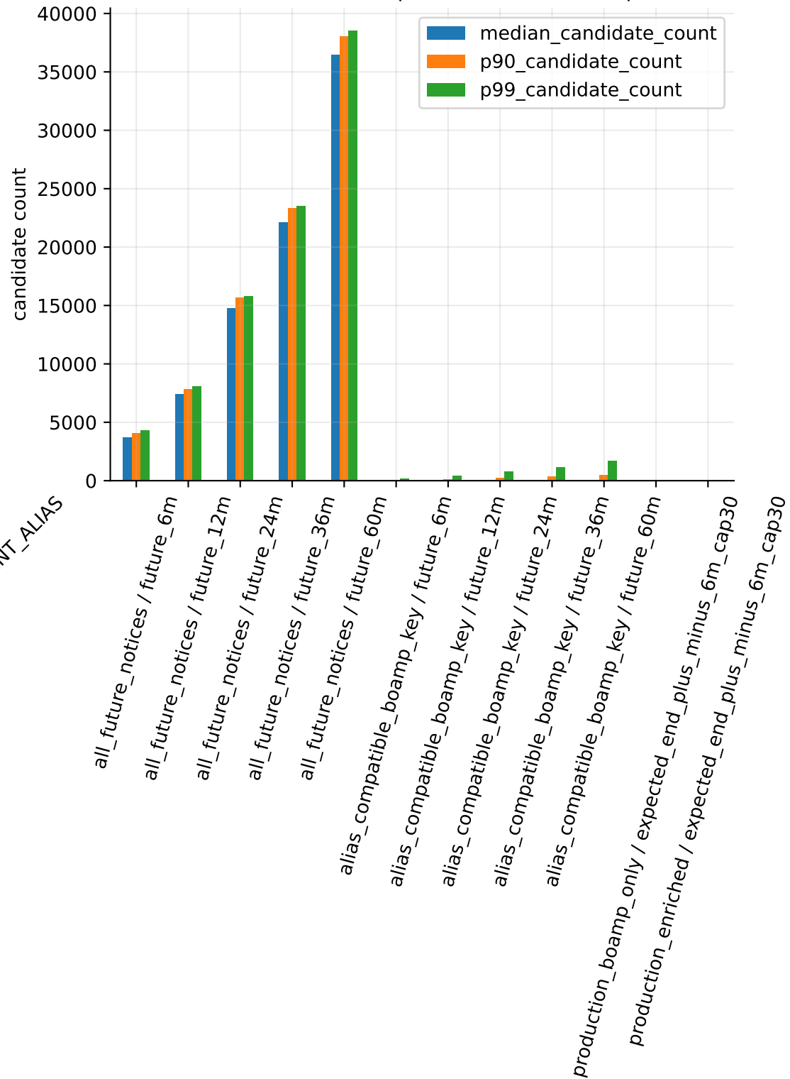
Ambient vs filtered vs production candidate pools
