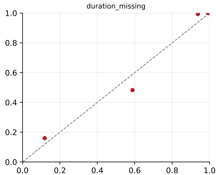
Observed vs. predicted probability (decile bins, L2-penalized logistic model), per flag
