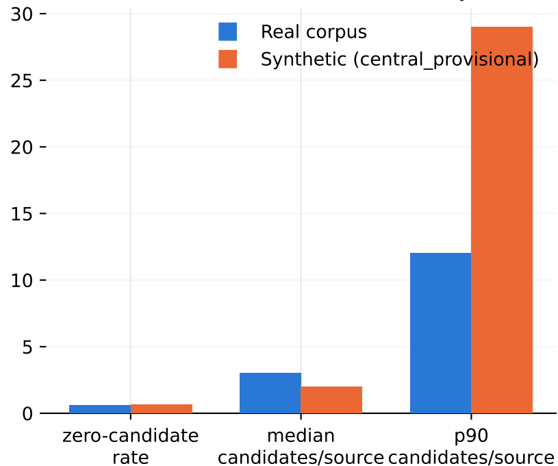
Candidate-environment summary
