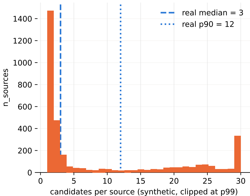
Candidate-count distribution
