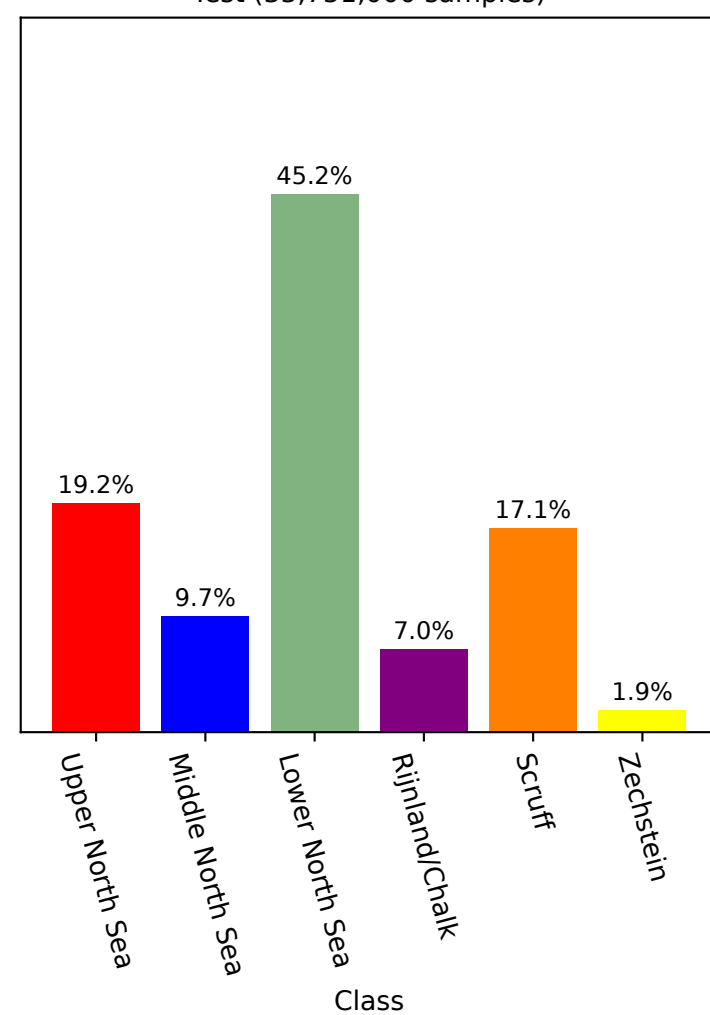
Test (35,751,000 samples)
