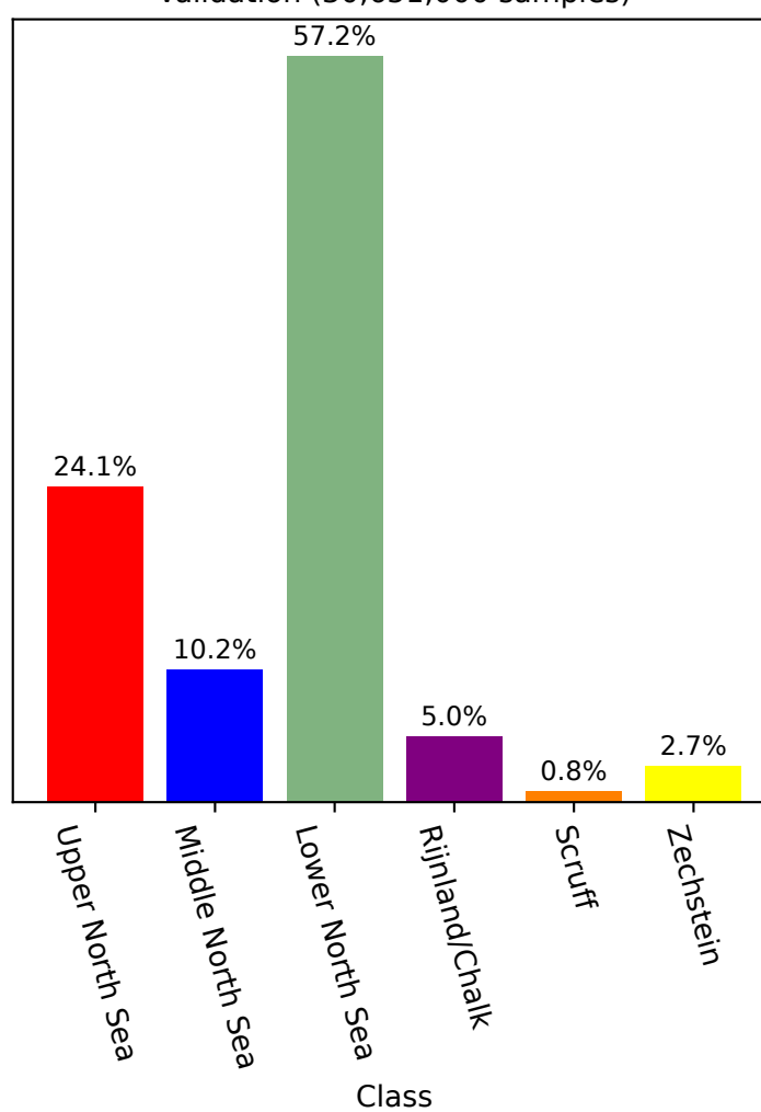
Validation (30,651,000 samples)
