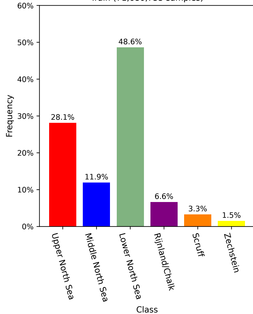
Train (71,680,755 samples)
