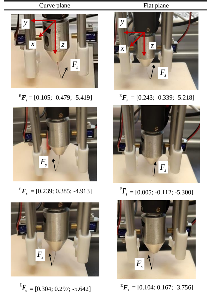
Fig. E.1 Force and bending degree of needle tip on flat and curved tissues
