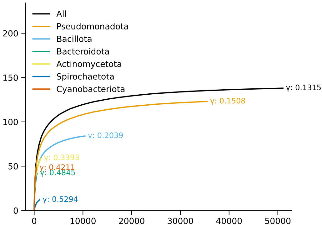
DS: type
