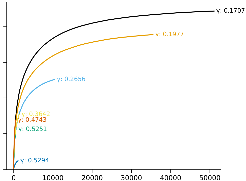
DS: subtype
