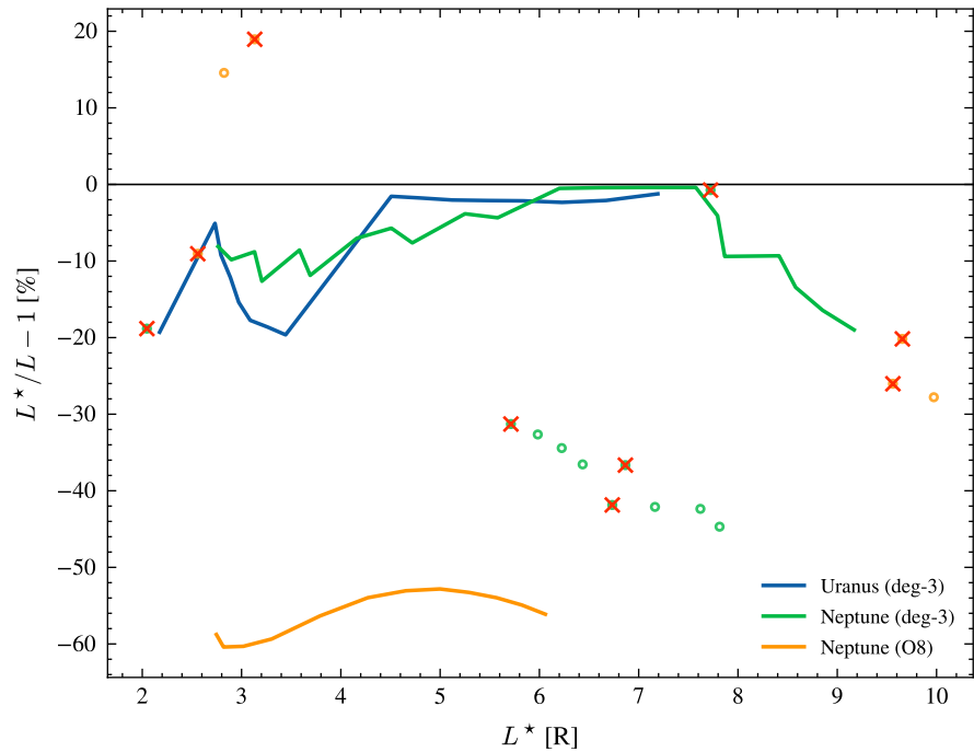
(b) dipole-L failure; x: fold points ( J=0 )
