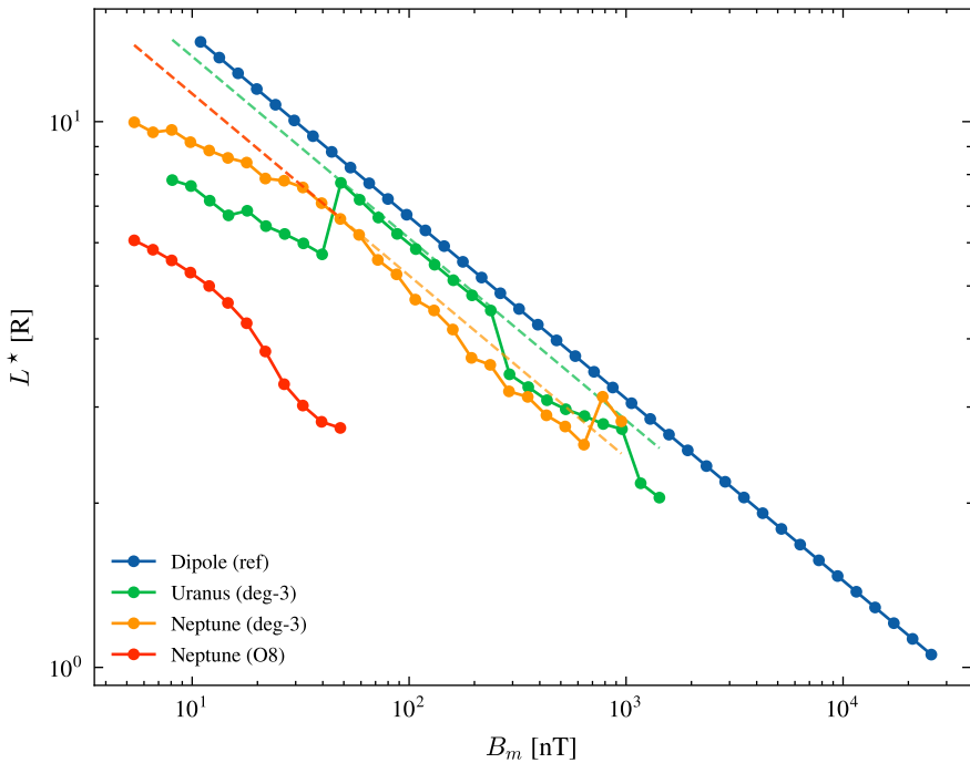
(a) L^*(B_m) tables; dashed: dipole reference L
