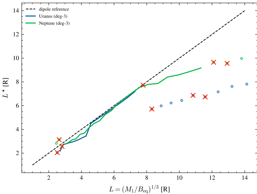
(c) remapped D : suppression at fold-adjacent L^*
